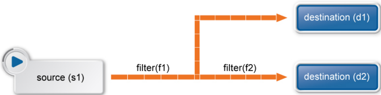
Figure 8.1. Embedded log statement
